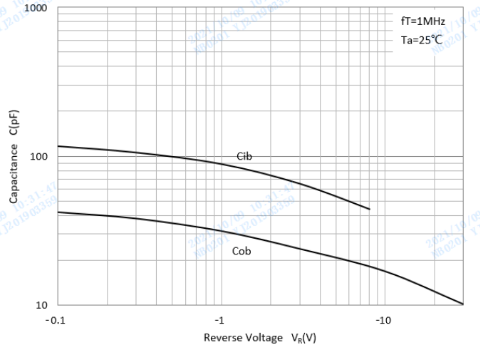
Cob/Cib-V CE /V EB
